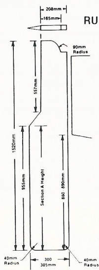
Section A showing stations measured from leading edge.
